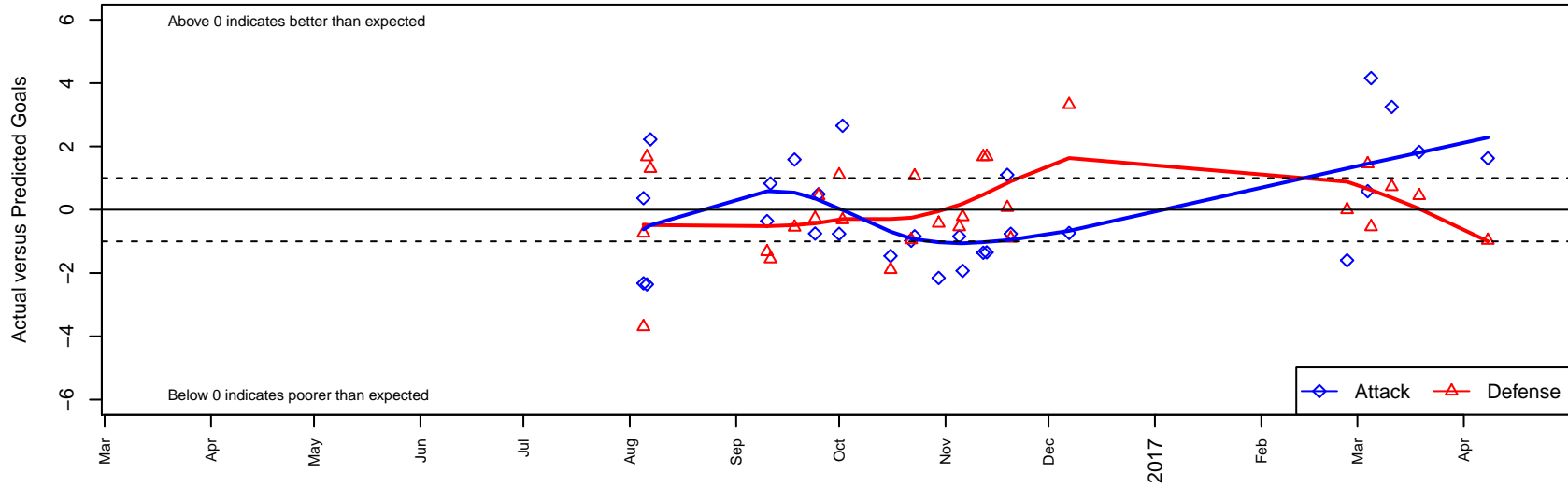
FSC Roses White G05 Dots are actual minus expected GF (blue circles) and GA (red triangles). Blue line is smoothed change in attack strength. Red is smoothed change in defense strength.
